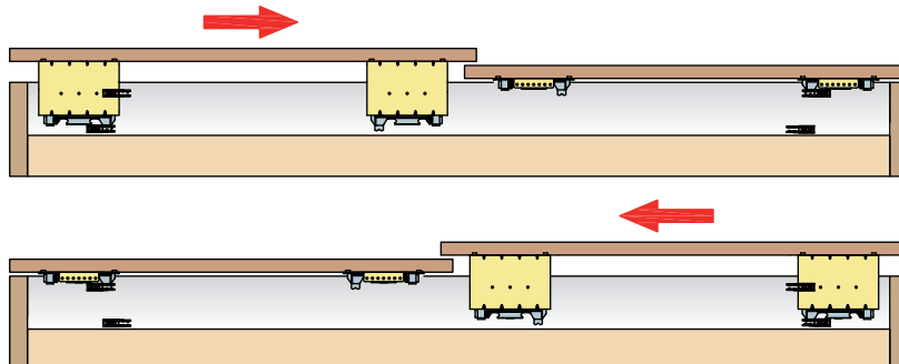
Armadio a 2 ante con 4 fermi a pinza in apertura e in chiusura Wardrobe with 2 doors, 4 classic stopper for opening and closing
